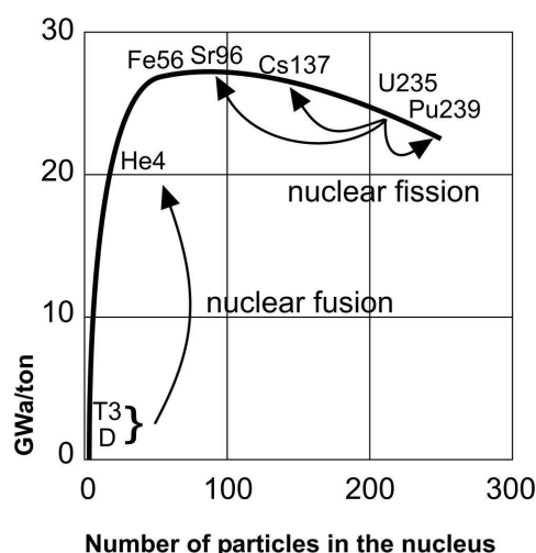
Fig. 20 Bond energy of nuclei as a function of the number of particles aa
