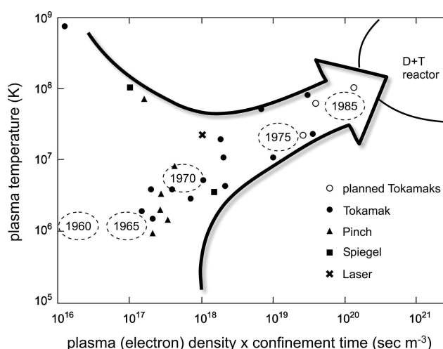
Fig. 21 Progress of nuclear fusion as expected in 1982 bb
