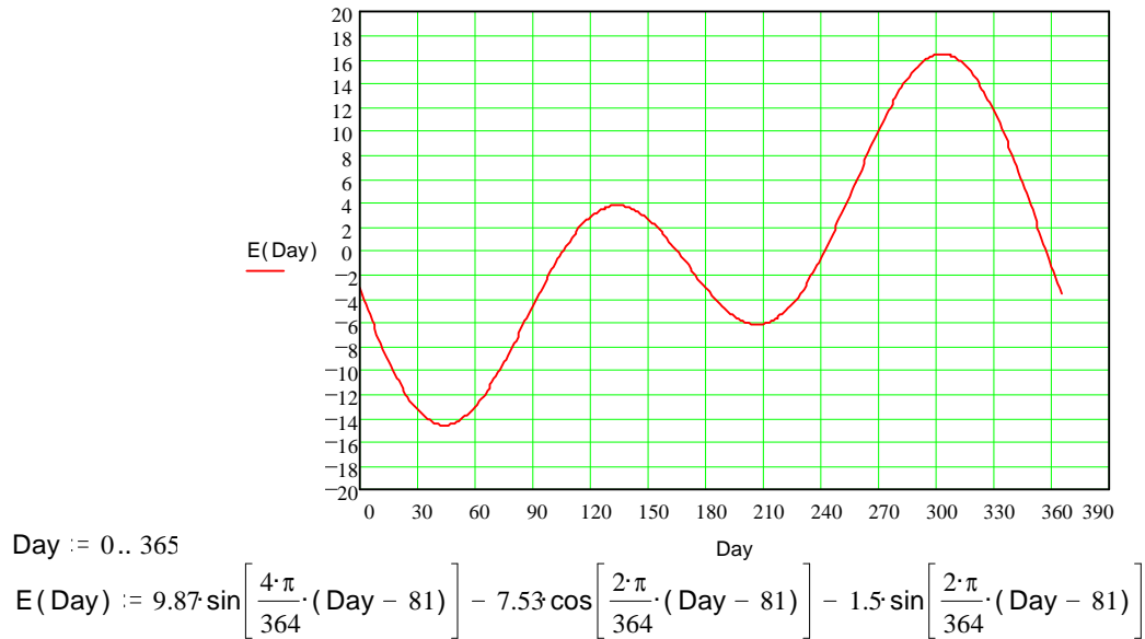
Fig. 43 Time equalization per day of the year
