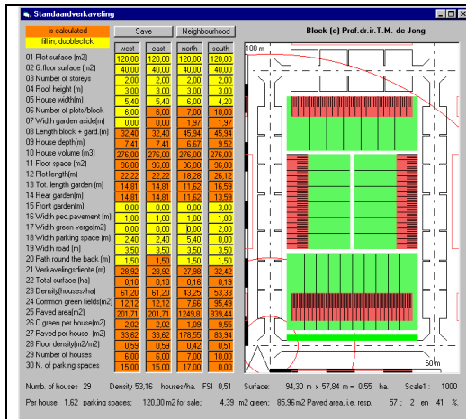
Fig. 51 Plot division taking shadow into account ss
