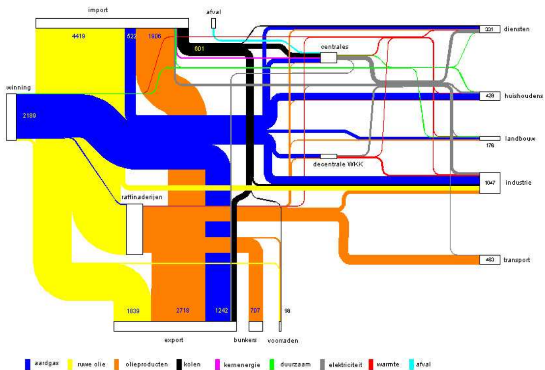
Fig. 31 Energy flows through The Netherlands, 2000 (x PJ or 31.7 MWh) kk
