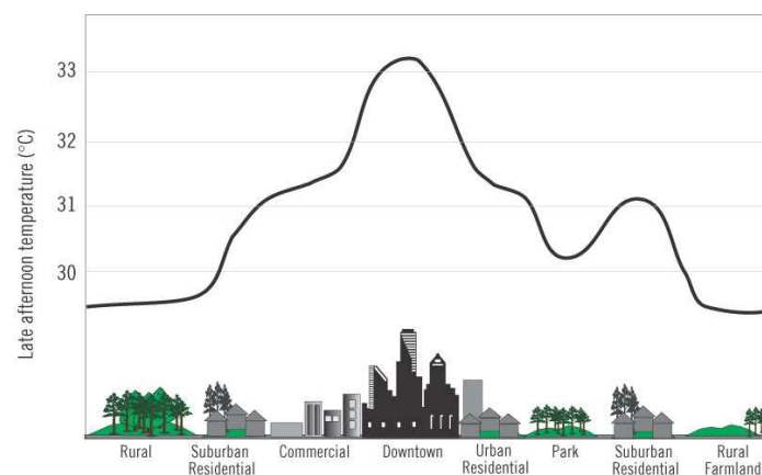
Fig. 67 The urban heat island aaa
