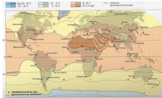
Fig. 62 Global summer temperatures xx
