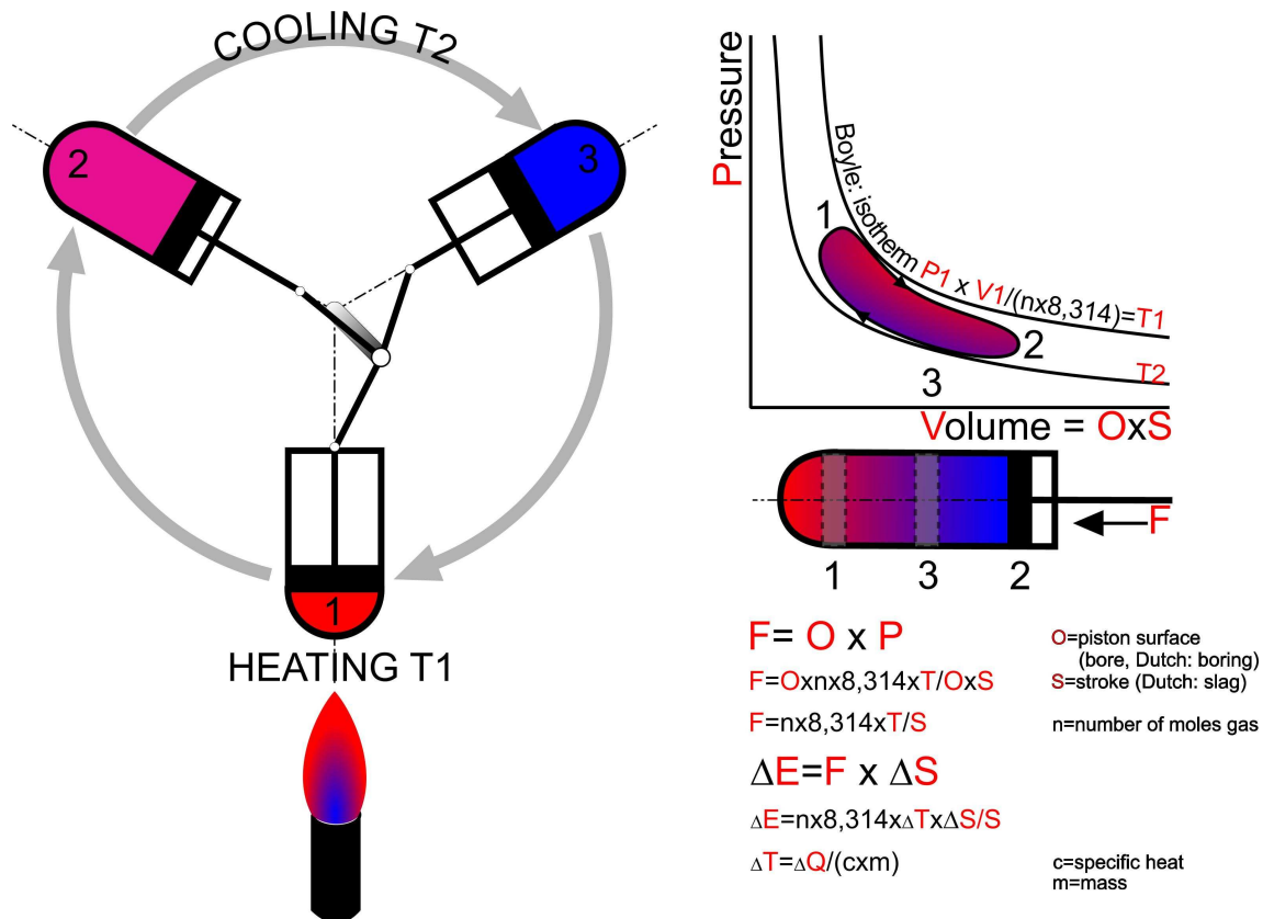
Fig. 12 Carnot-engine
