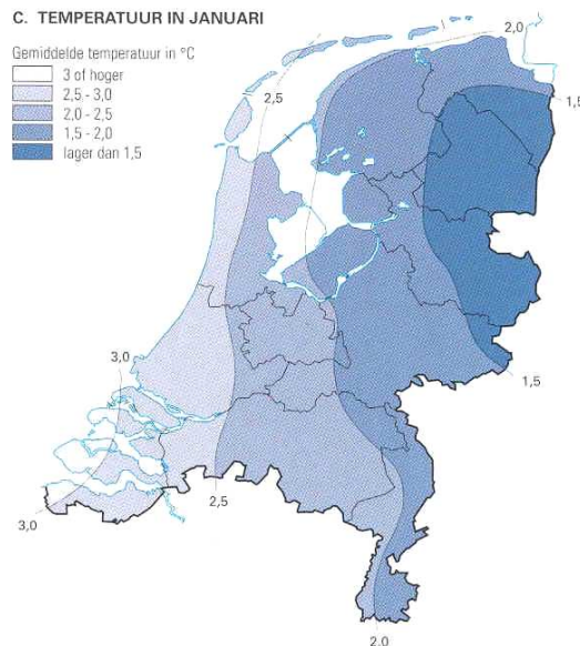
Fig. 65 Winter temperatures in the Netherlands
