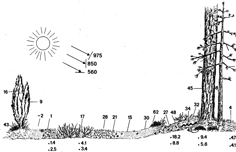
Fig. 69 Surface temperatures along a line perpendicular to edge of a forest bbb
