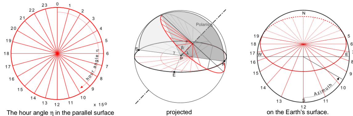
Fig. 40 The hour angle transformed into Azimuth.
