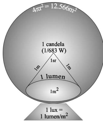
Fig. 59 Candela, lumen, lux
