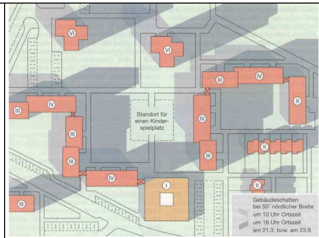
Fig. 52 Avoiding shadow by neighbours according to German regulations tt
