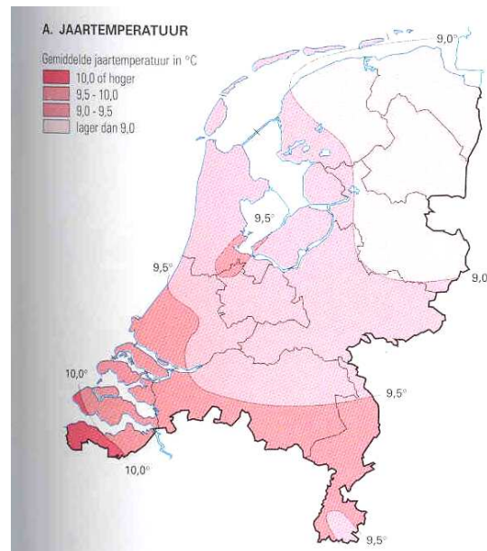
Fig. 66 Year temperatures in the Netherlands zz
