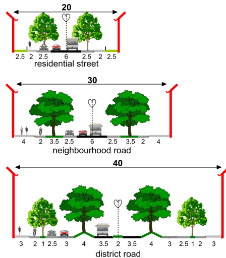
Fig. 542 Profiles normalised to 20, 30 and 40m
