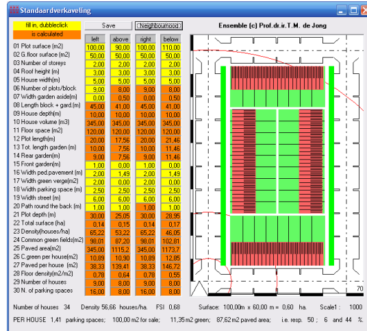
Fig. 540 Elongating and adapting 100x60m
