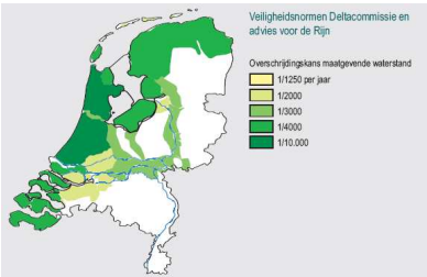
Source: Fig. 451 a Proposed changes of safety standards (MNP, 2004)
