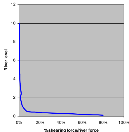
Fig. 381 The influence of shearing force by different water levels in Fig. 380 c
