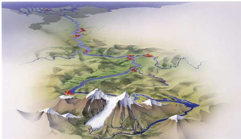
Fig. 361 The river basin of the Rhine (Paul Maas, opdrachtgever: Thieme Meulenhoff)
